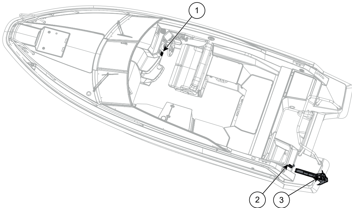
Figure 11.2 Yamarin 67 DC - Guindeau
